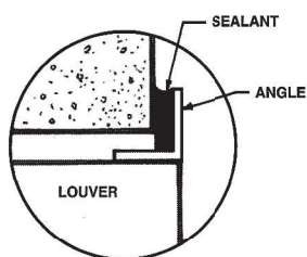
A LOUVER MUCH DEEPER THAN WALL
